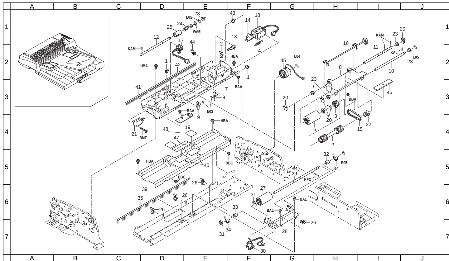
FIG. 4 PAPER FEED SECTION
