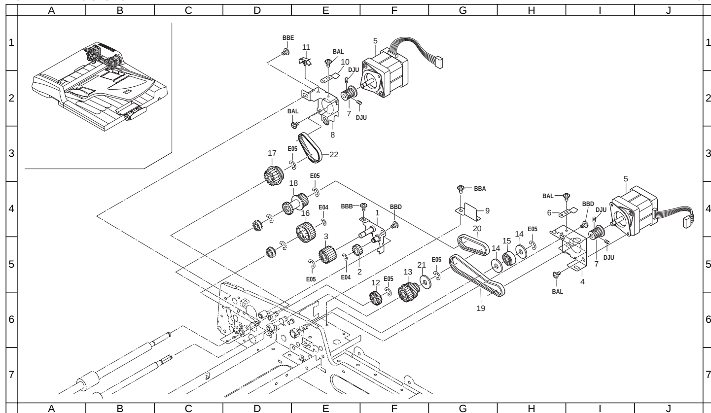
FIG. 7 DRIVING SECTION
