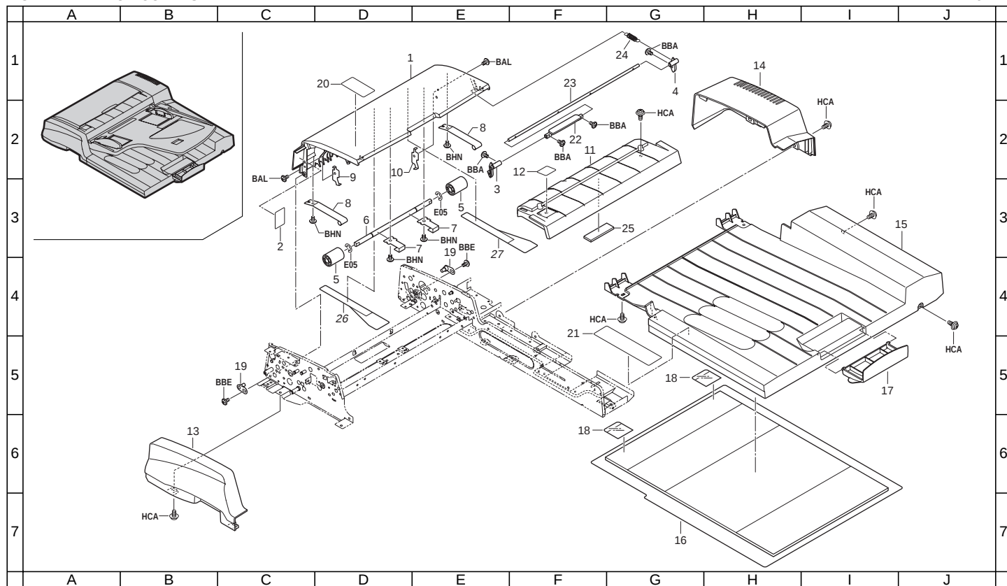
FIG. 1 EXTERIOR COVERS
