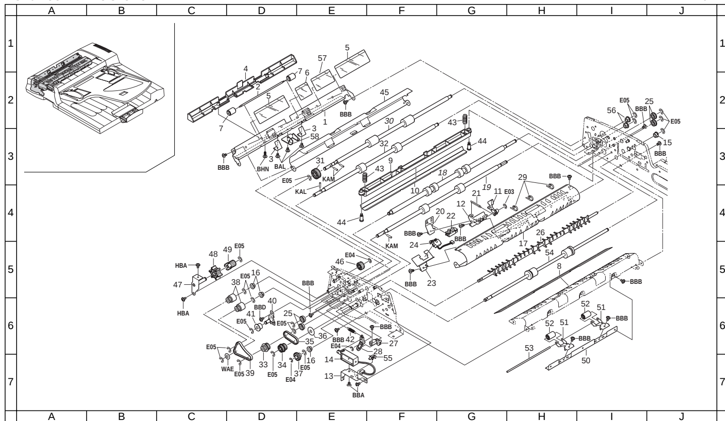
FIG. 6 CONVEYING SECTION
