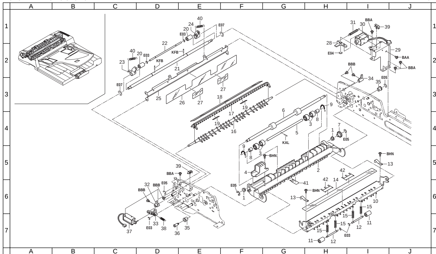
FIG. 5 REVERSING SECTION
